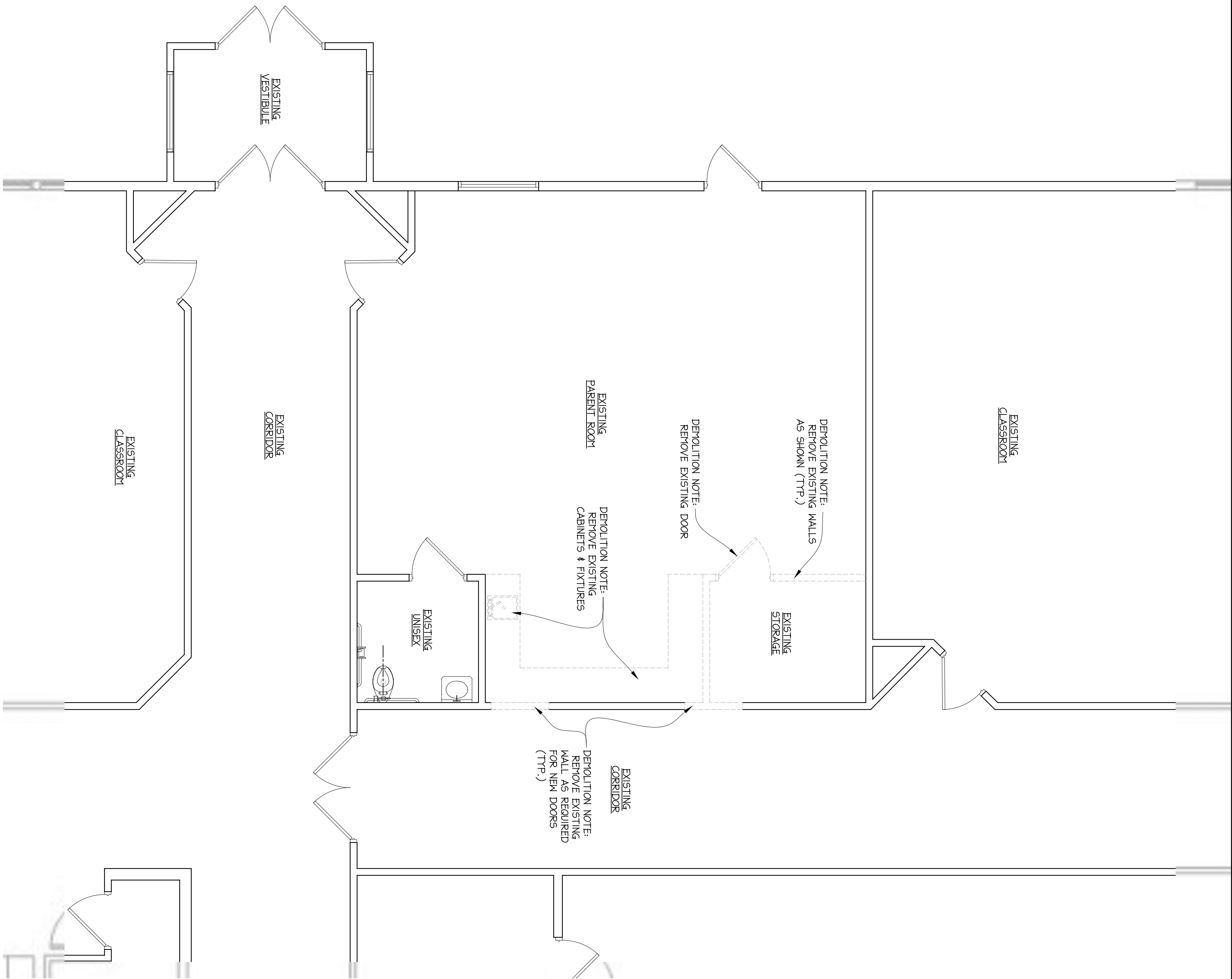
N ENLARGED EXISTING/ DEMOLITION FLOOR PLAN SCALE: 1/4" = 1'-0"
